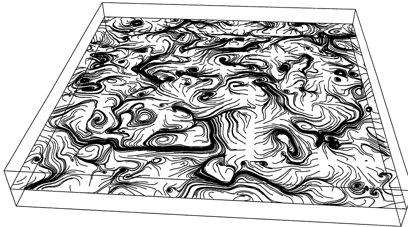
TRANS: Ra=1.E+7; 260
