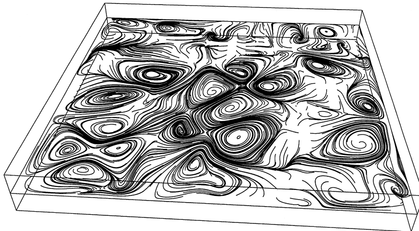
Fig. 7. Instantaneous trajectories of massless particles in the central horizontal plane for one DNS ( Ra = 6.5 \times 10^5 ) and one TRANS realisation ( Ra = 10^7 ).
